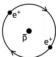
anti-hydrure \bar{H}^+ Stable
